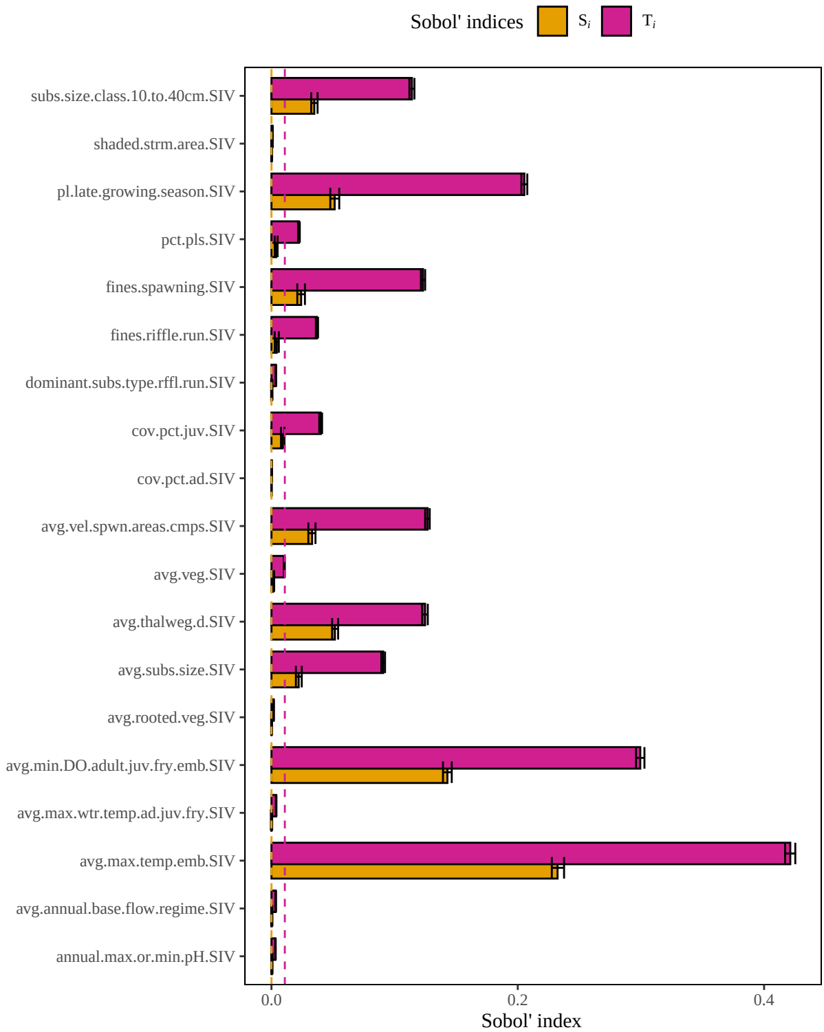
Figure 3. Results of a sensitivity analysis for the cutthroatRivGenMt15CLtoe5m model based on the original author-specified model outlined in Hickman and Raleigh (1982). Dashed lines represent baseline numerical approximation error for S_i and T_i ( i.e. , dummy variables).
